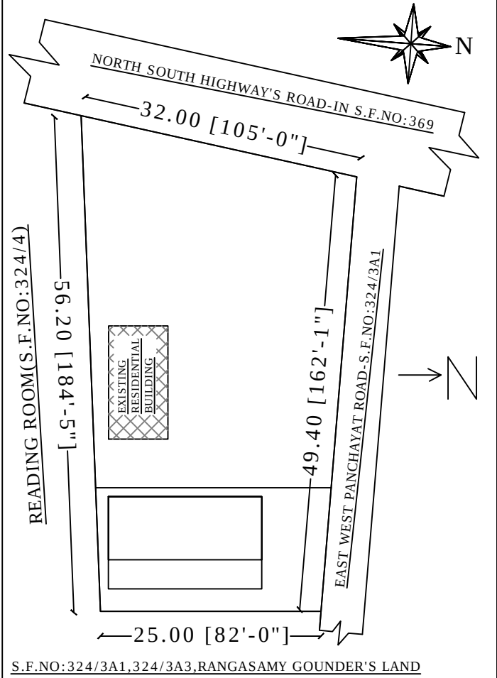
S.F.NO:324/3A1,324/3A3,RANGASAMY GOUNDER'S LAND
