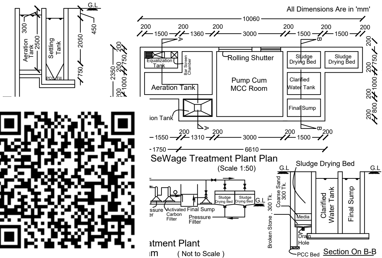
Plan of SeWage Treatment Plant & Hydraulic FloW Diagram
