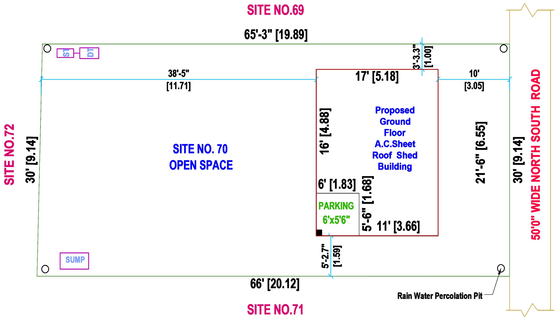
SITE PLAN (SCALE 1" : 8' 0")
