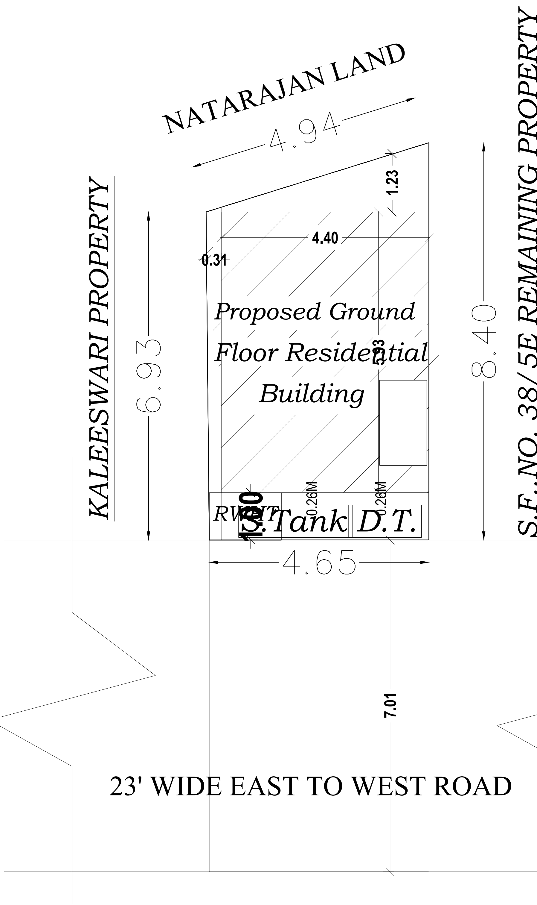
SITE PLAN
