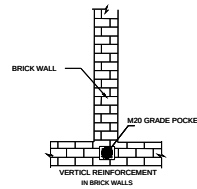
VERTICAL REINFORCEMENT IN BRICK WALLS
