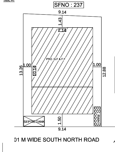
TRIAL PIT
