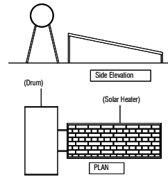
Solar Water Heater Details (Not to scale)
