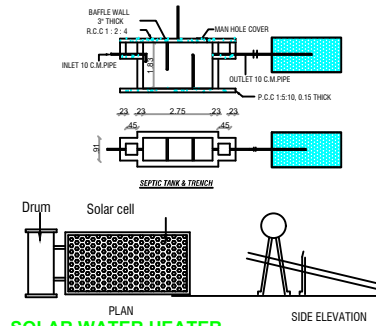
SOLAR WATER HEATER DETAILS (NTS)
