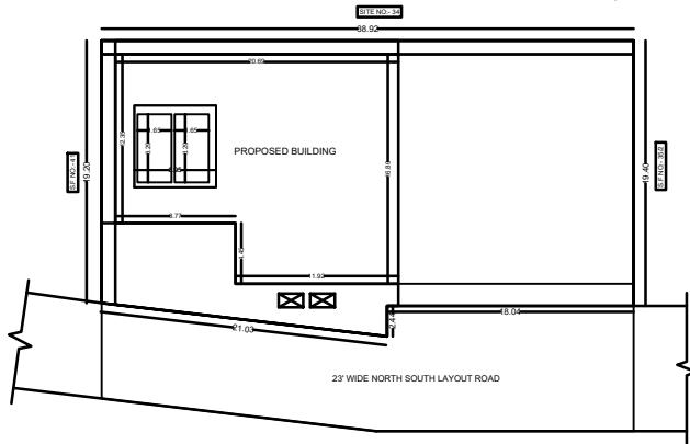
SITE PLAN
