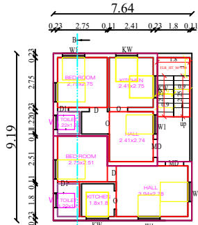
PRO.S.FLOOR PLAN
