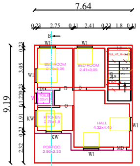
EXTG.G.FLOOR PLAN
