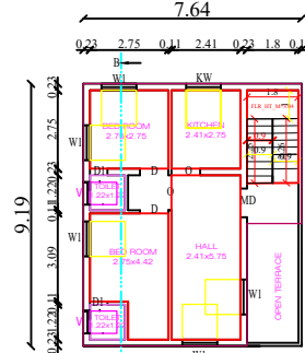
PRO.S.FLOOR PLAN
