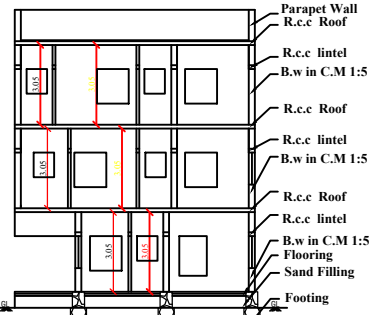
SECTION AB
