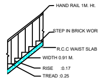
STAIR DETAIL
