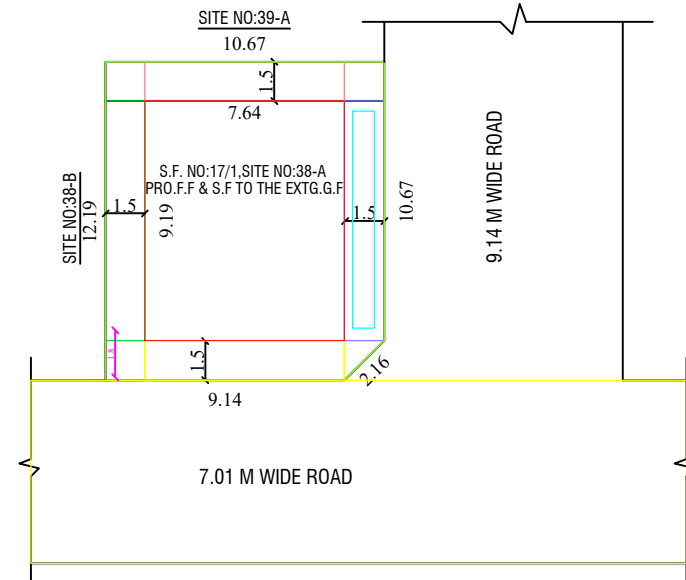
SITE PLAN
