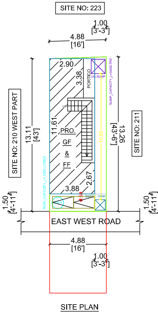
SITE PLAN
