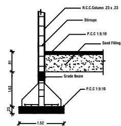
COLUMN DETAIL
