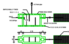
SEPTIC TANK AND TRENCH
