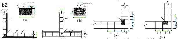
Figure - 2 : Typical Details of Providing Vertical Steel Bars in Brick Masonry.
