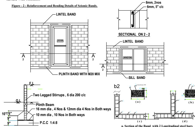
Figure 2: Reinforcement and Bending Details of Seismic Bands.
