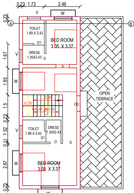
PROPOSED FIRST FLOOR BUILDING
