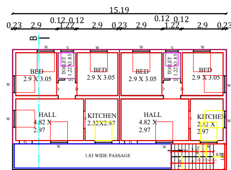
PRO.F.FLOOR PLAN
