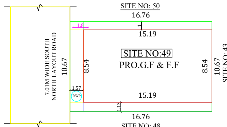
SITE PLAN
