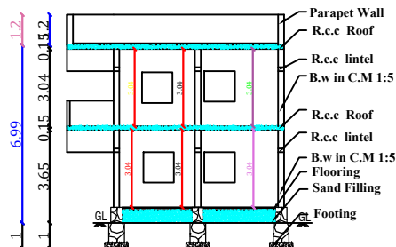
SECTION AB
