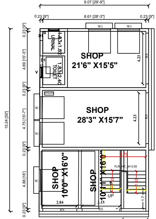
PROPOSED GROUND FLOOR SHOP PLAN
