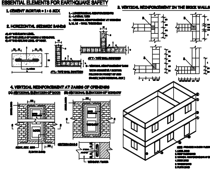
ESSENTIAL ELEMENTS FOR EARTHQUAKE SAFETY
