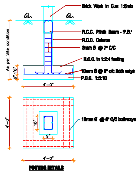
FOOTINGS DETAILS
