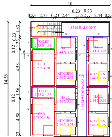
F.FLOOR PLAN
