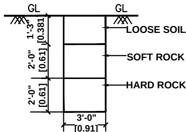
TRAIL PIT (NOT TO SCALE)
