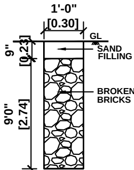
SECTION 1 - 1
