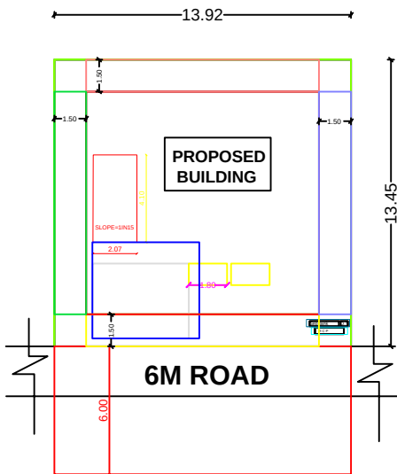
SITE PLAN
