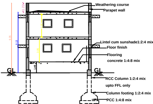
SECTION ELEVATION
