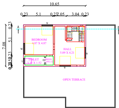
PRO-FIRST FLOOR
