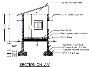
SECTION ON-AA'
