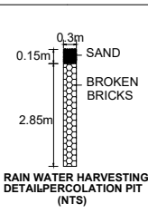
RAIN WATER HARVESTING DETAIL PERCOLATION PIT (NTS)
