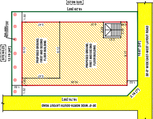
SITE PLAN
