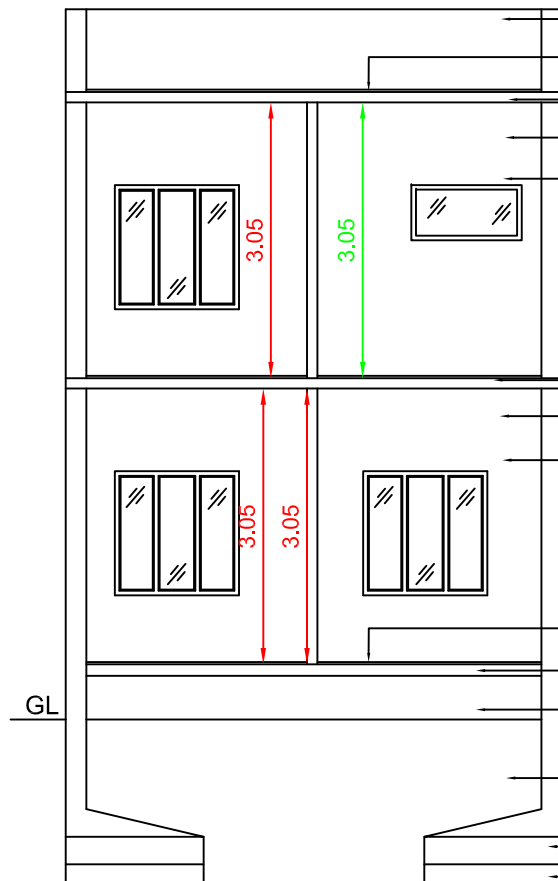
CROSS SECTION ON XY
