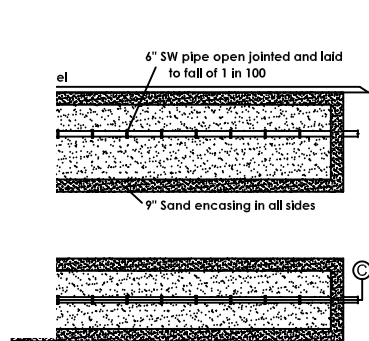
SEPTIC TANK (NTS)
