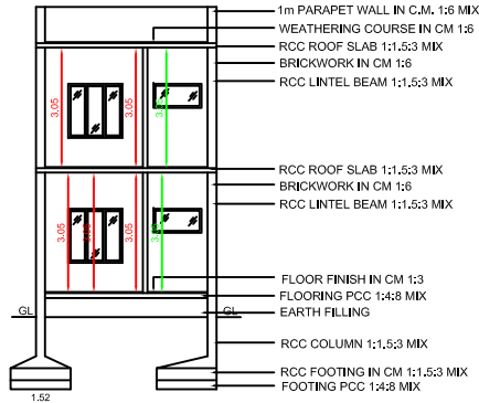
CROSS SECTION ON XY
