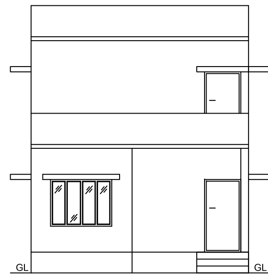
FRONT ELEVATION
