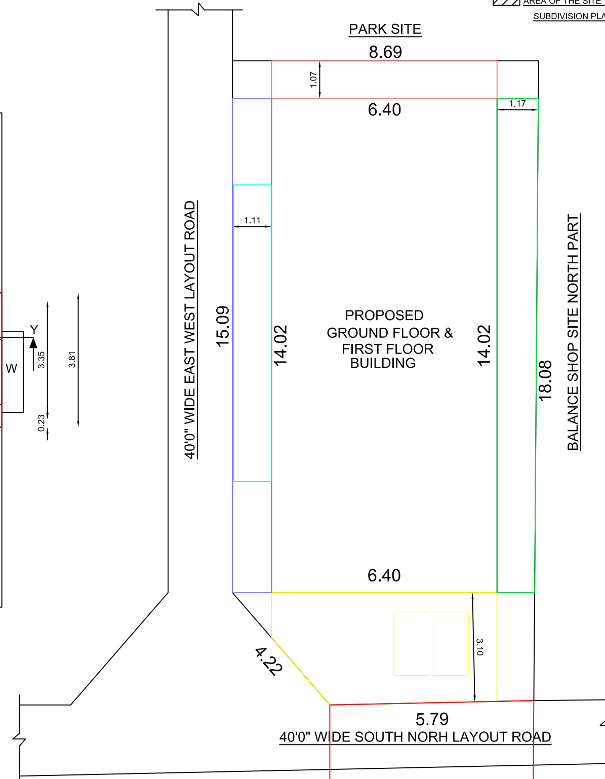
SITE PLAN
