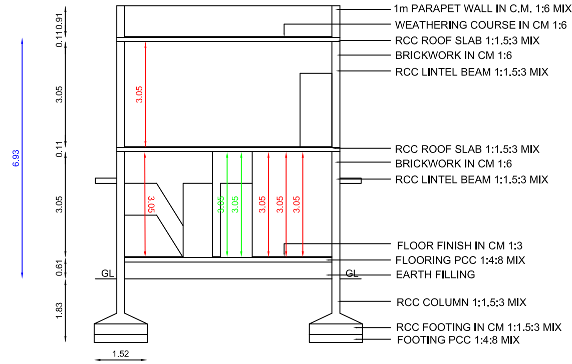
CROSS SECTION ON XY
