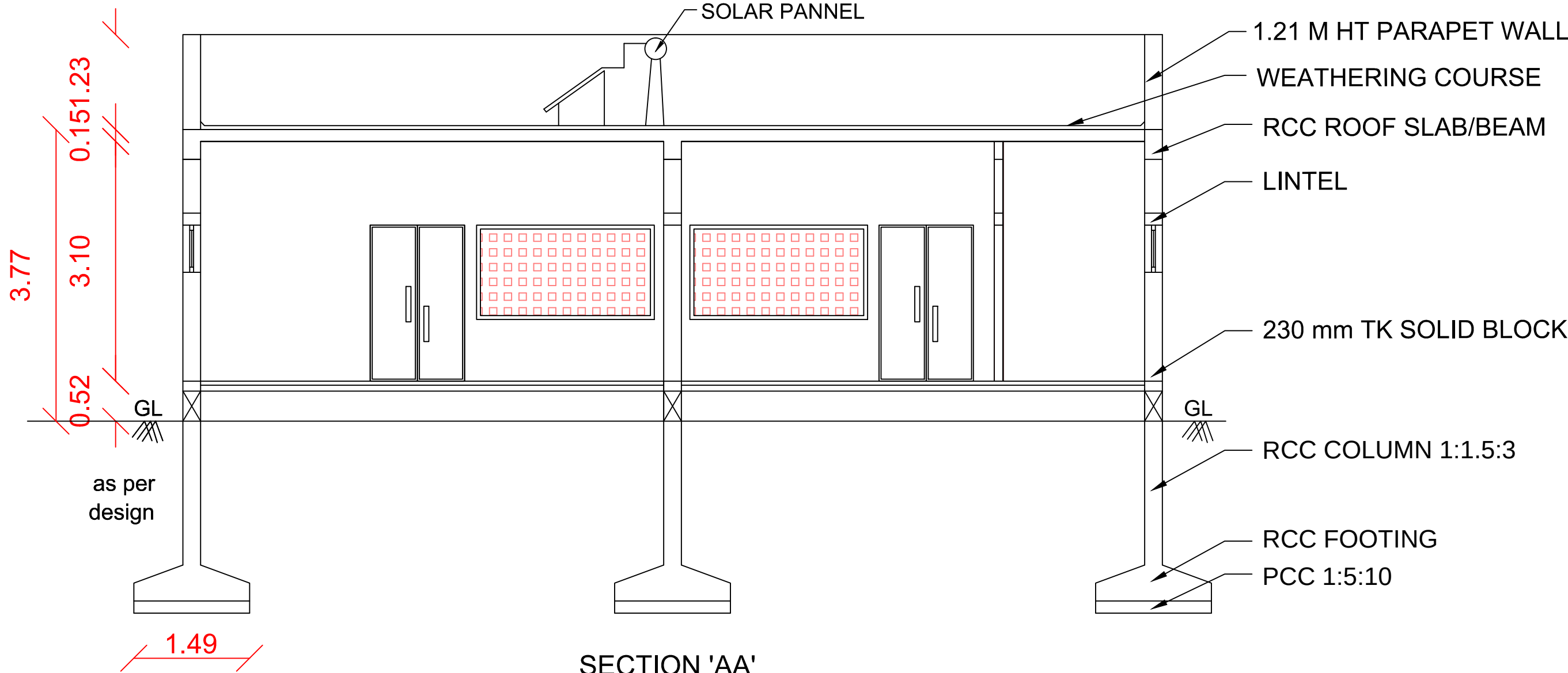
SECTION 'AA'
