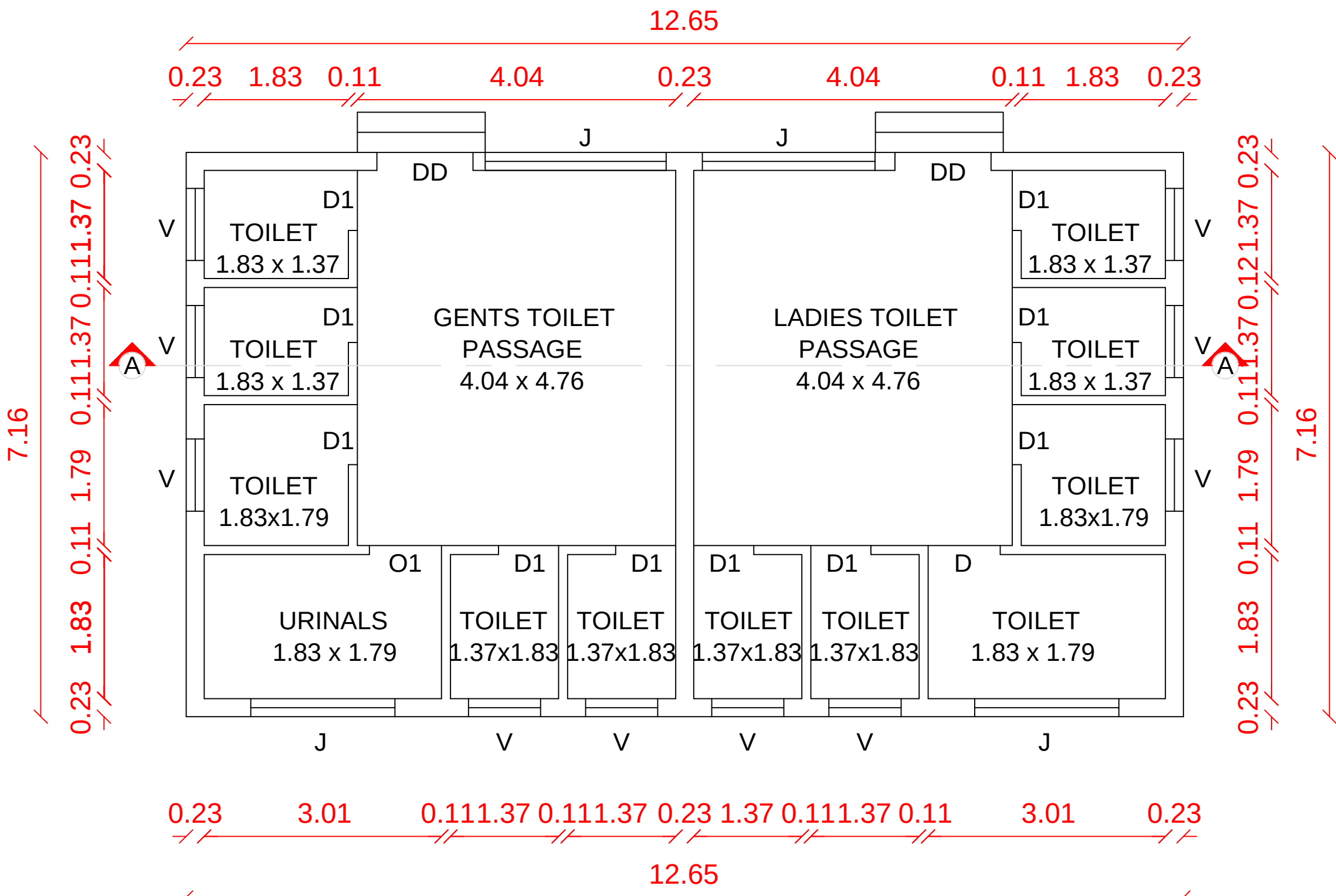
BLOCK No - 02 EXISTING TOILET BUILDING GROUND FLOOR PLAN
