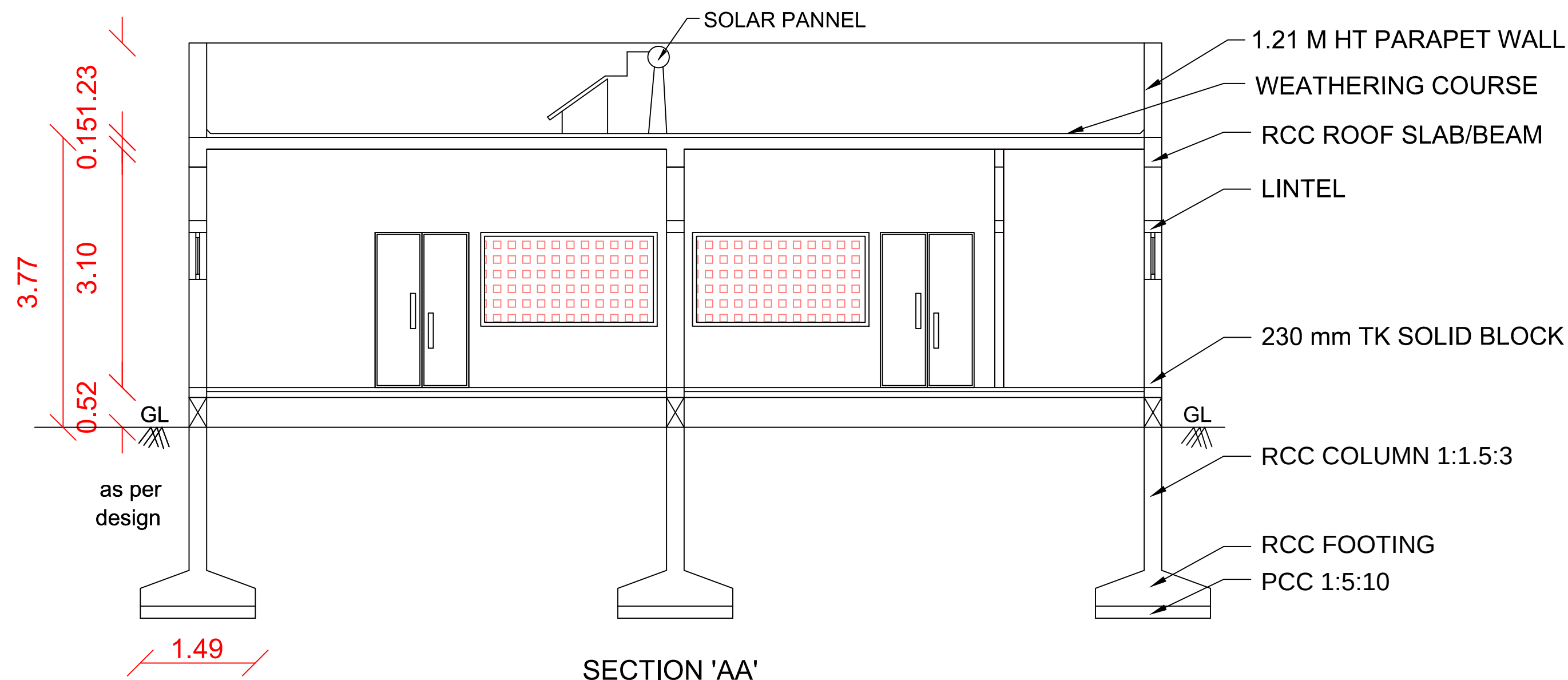
SECTION 'AA'
