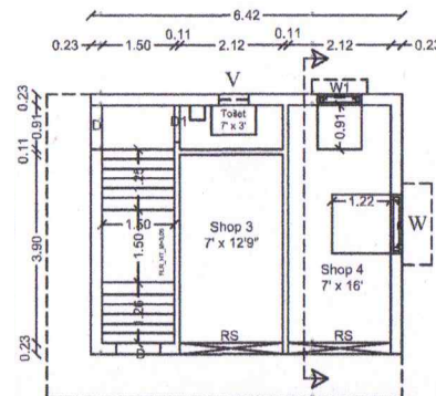
Revised First Floor Plan
