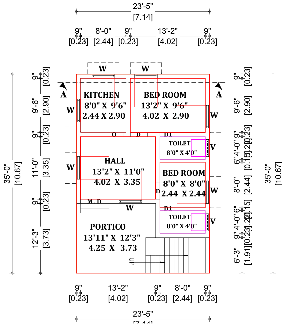
D FLOOR PLAN
