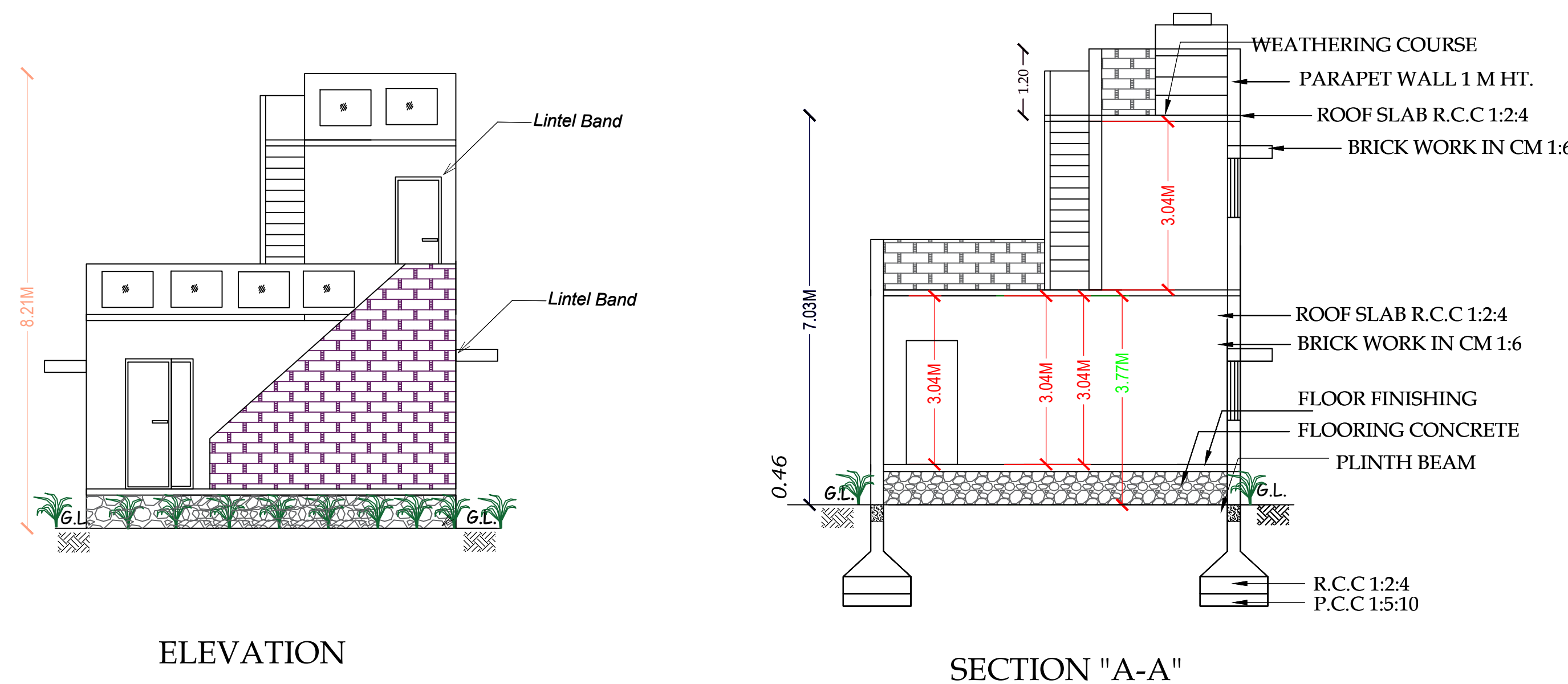
SECTION "A-A"
