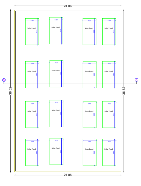
GROUND FLOOR TERRACE PLAN
