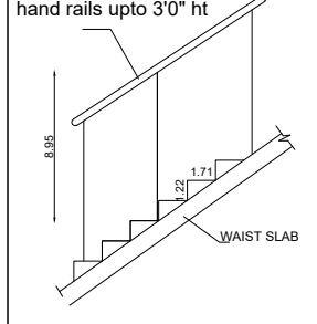
Hand rails upto 3'0" ht
