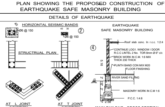
PLAN SHOWING THE PROPOSED CONSTRUCTION OF EARTHQUAKE SAFE MASONRY BUILDING
