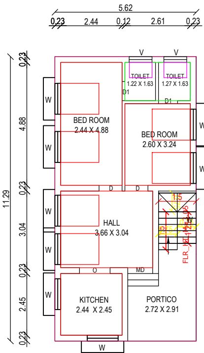
PROPOSED GROUND FLOOR BUILDING
