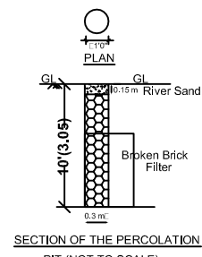
SECTION OF THE PERCOLATION PIT (NOT TO SCALE)
