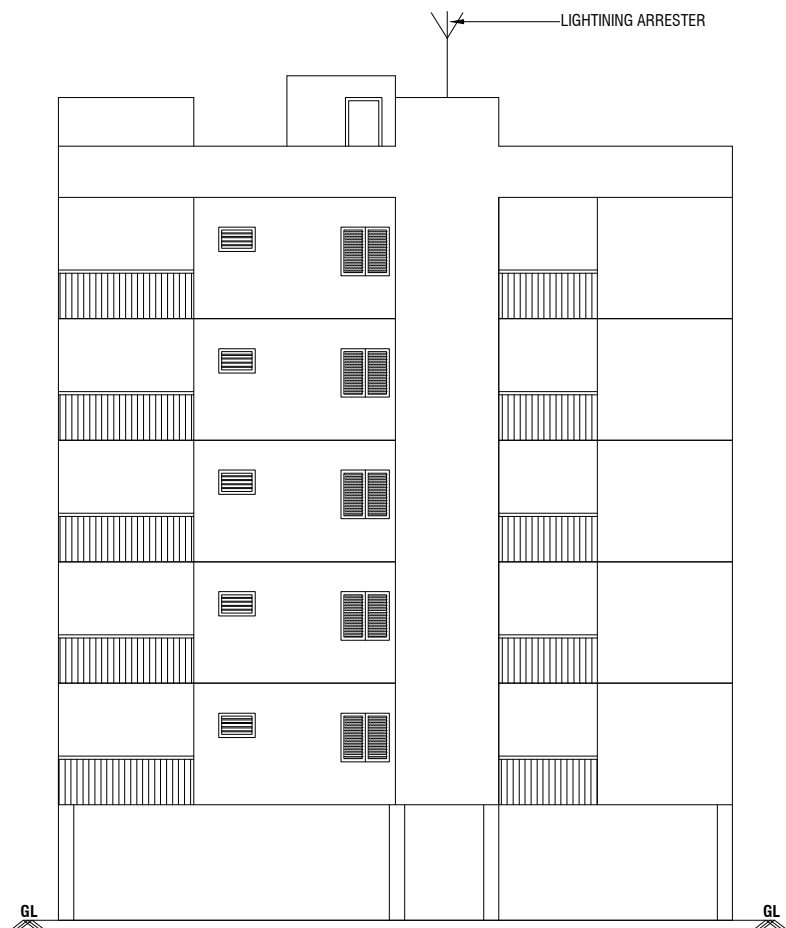
ELEVATION @ NORTH SIDE
