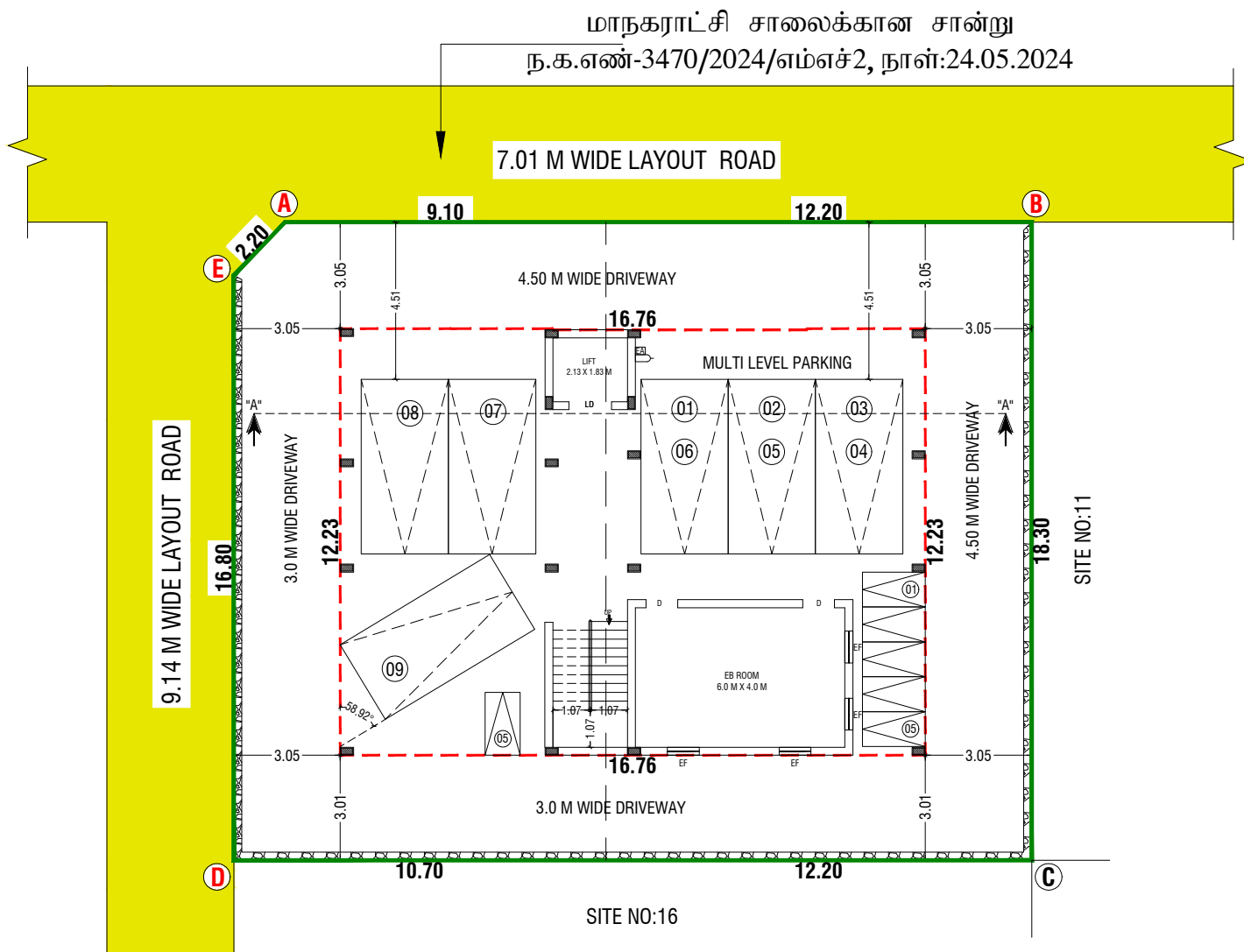
STILT FLOOR PLAN
