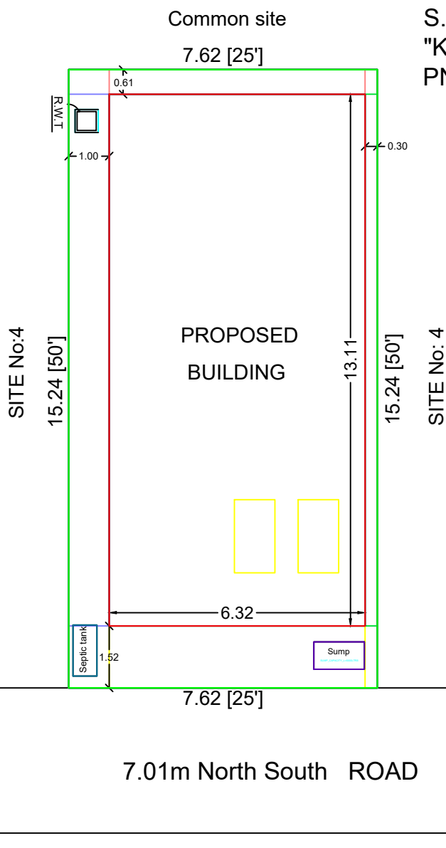
SITE PLAN
