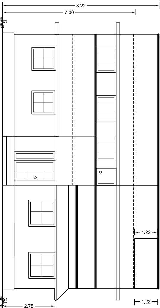
Elevation (East - Facing)
