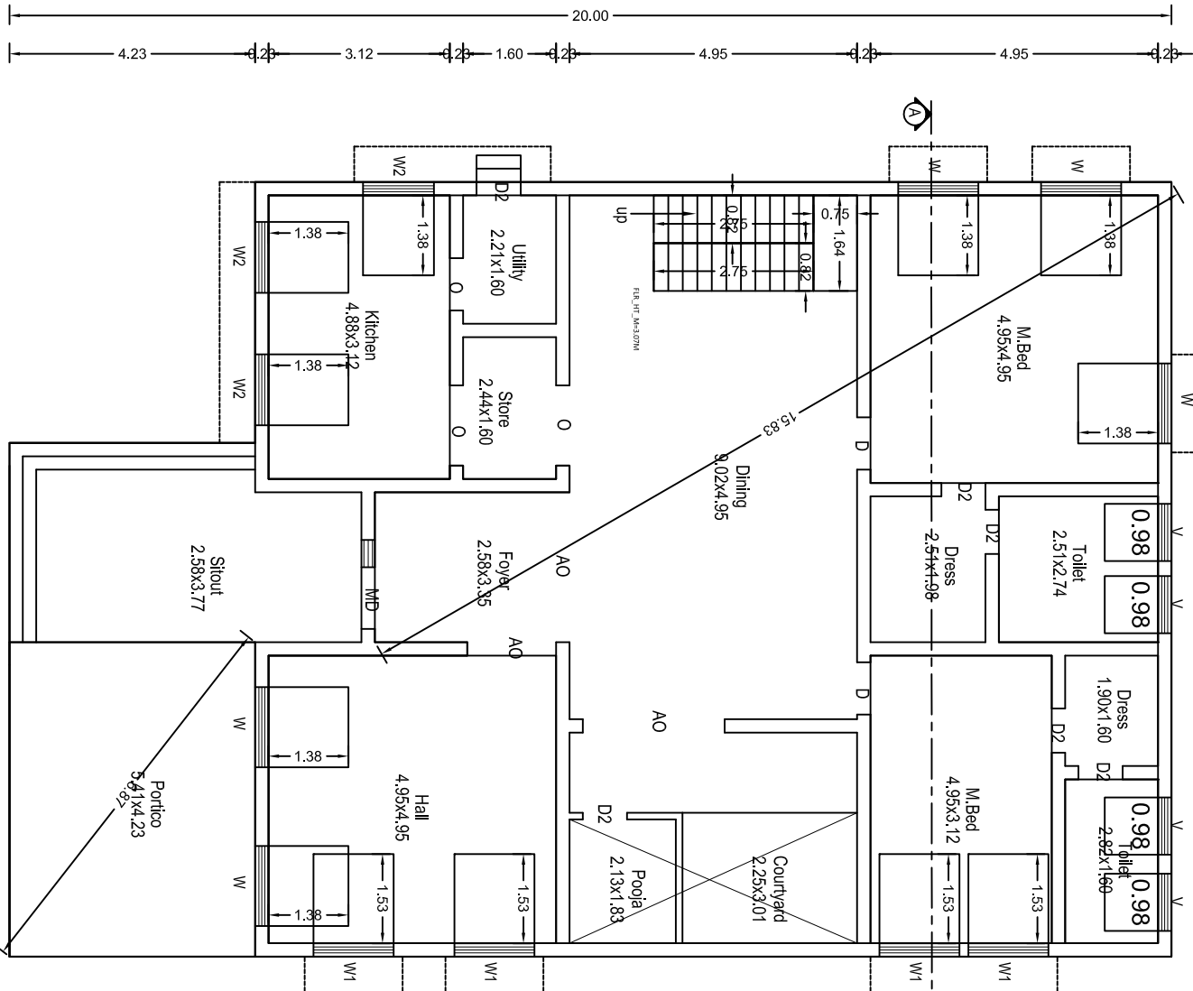
Plan Scale 1:100 Ground floor
