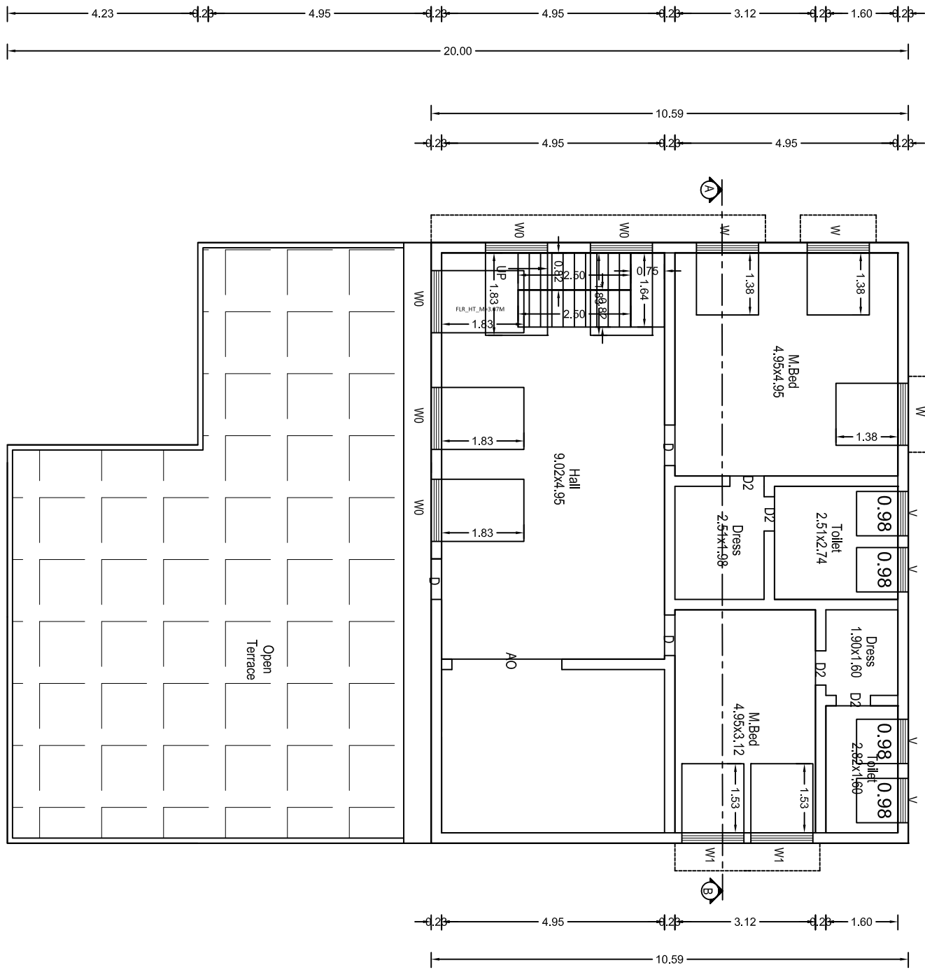
Plan Scale 1:100 First floor
