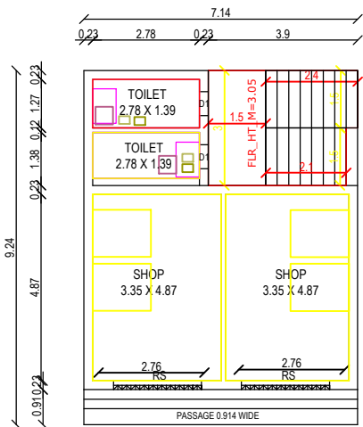
PROPOSED GROUND FLOOR BUILDING
