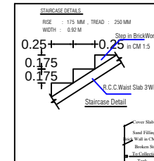
STAIRCASE DETAILS
