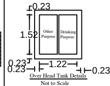
Over Head Tank Details
