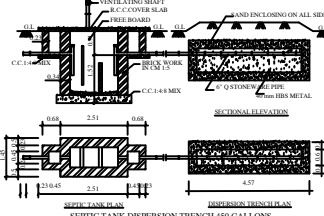
SEPTIC TANK DISPERSION TRENCH 450 GALLONS
