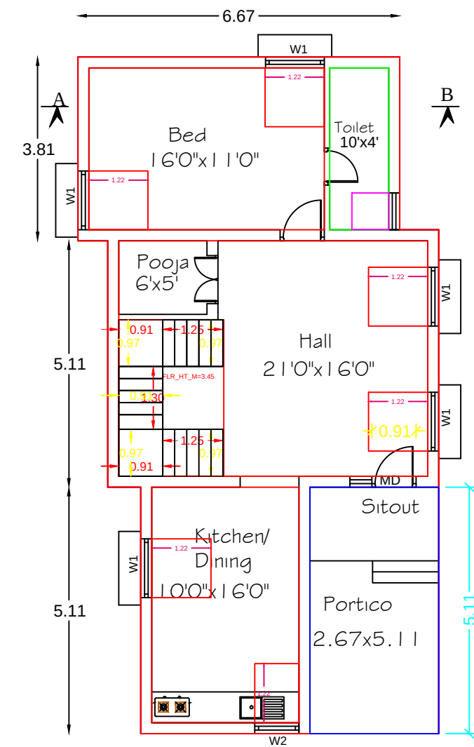
FLOOR PLAN
