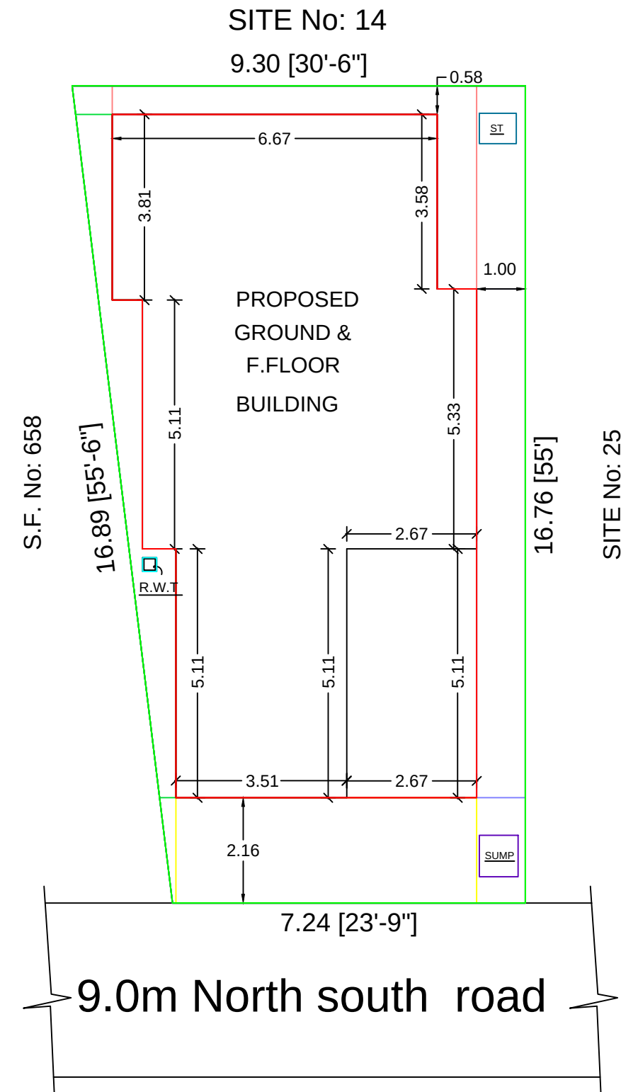
SITE PLAN
