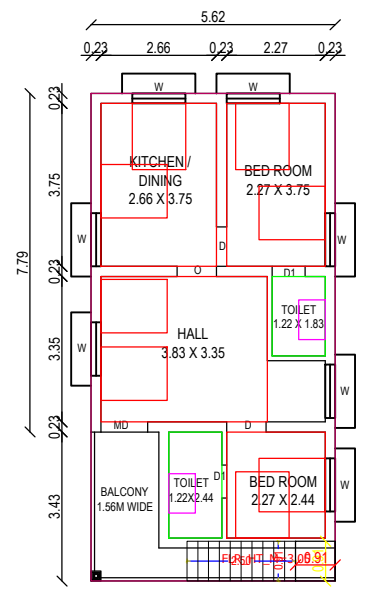
PROPOSED FIRST FLOOR BUILDING
