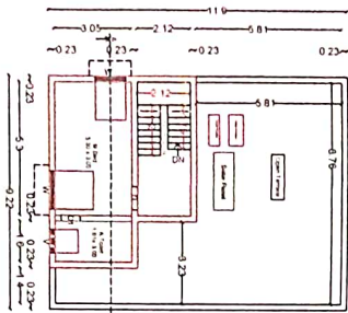
PROPOSED FIRST FLOOR PLAN SCALE 1:100
