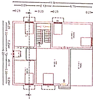
PROPOSED GROUND FLOOR PLAN SCALE 1:100
