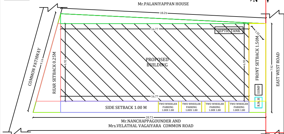
SITE PLAN :-
