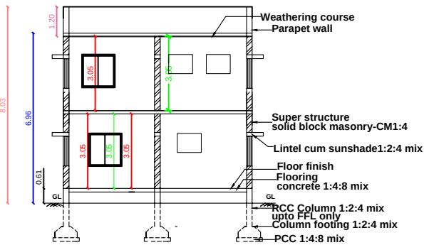
SECTION ELEVATION
