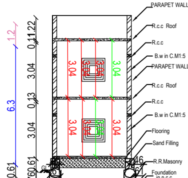
SECTION ,AB
