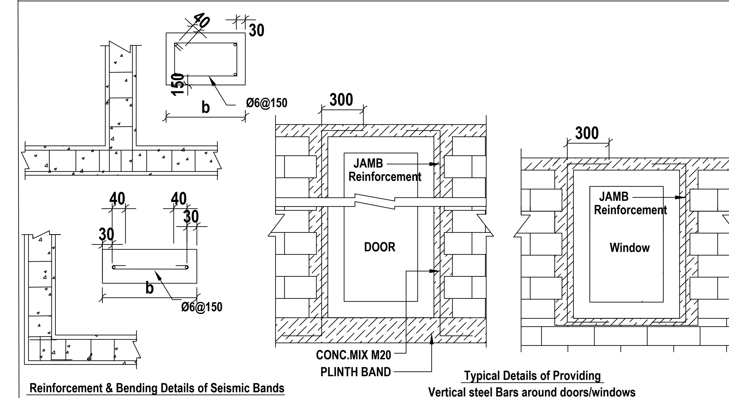
Essential Internal Elements in Building for Earthquake safety
