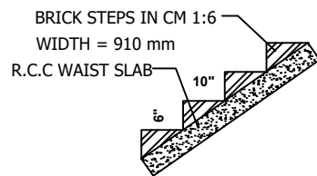
STAIRCASE DETAILS (NOT TO SCALE)
