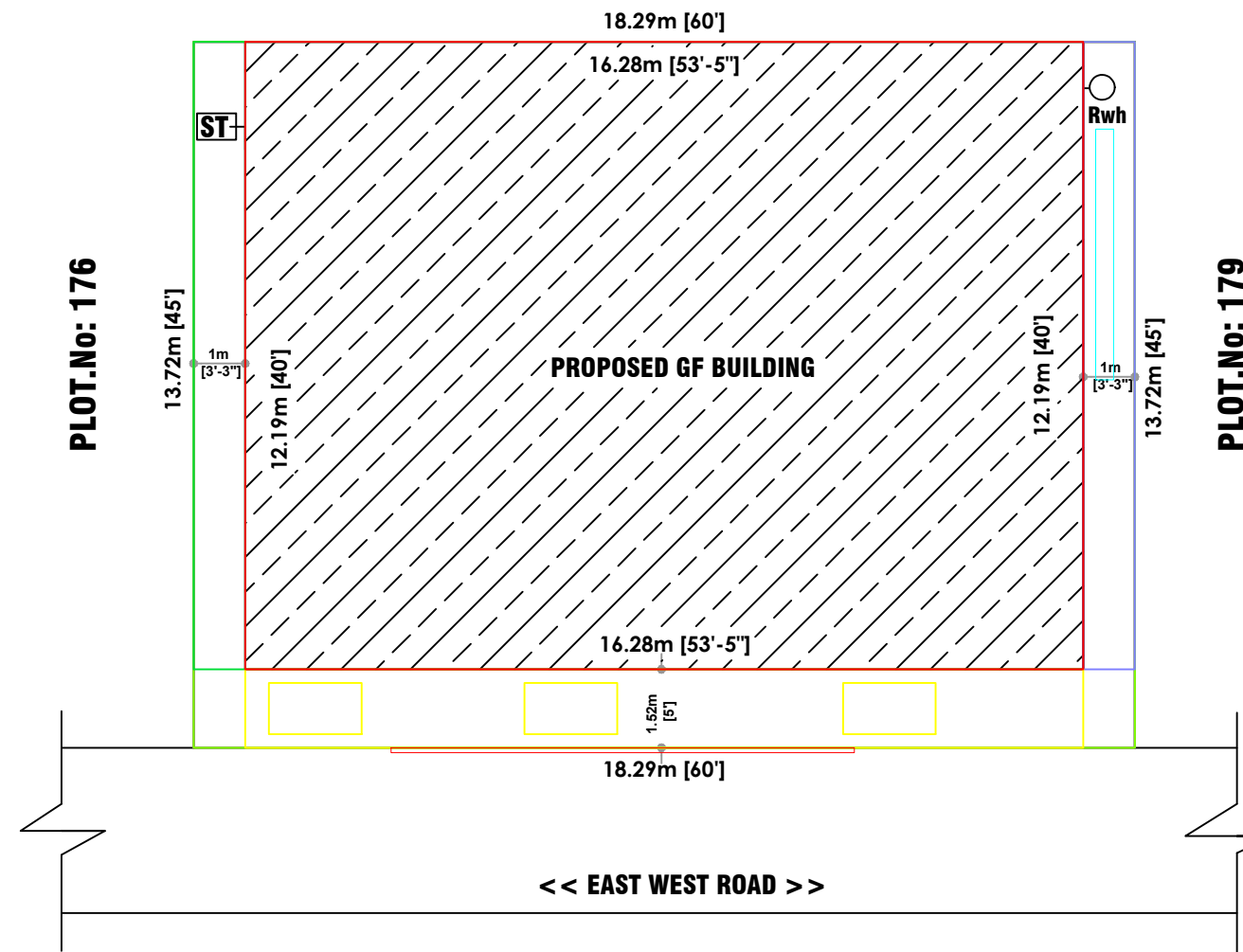
SITE PLAN
