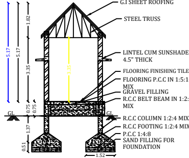
BLOCK 2 SECTION A-B
