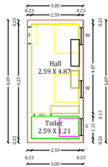
BLOCK 2 GROUND FLOOR PLAN
