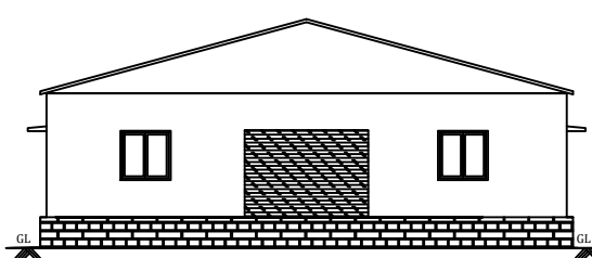
BLOCK 1 ELEVATION
