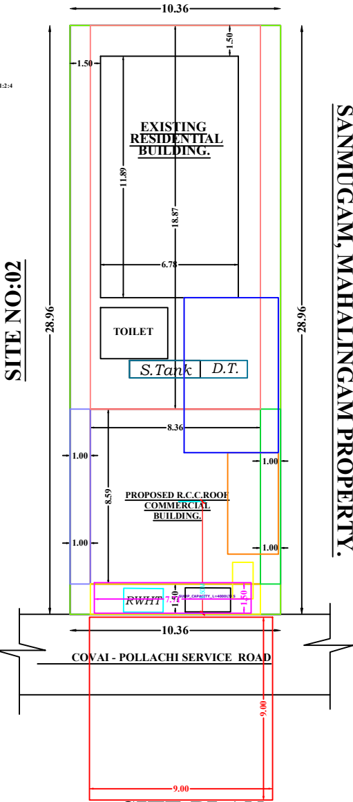
SITE PLAN
