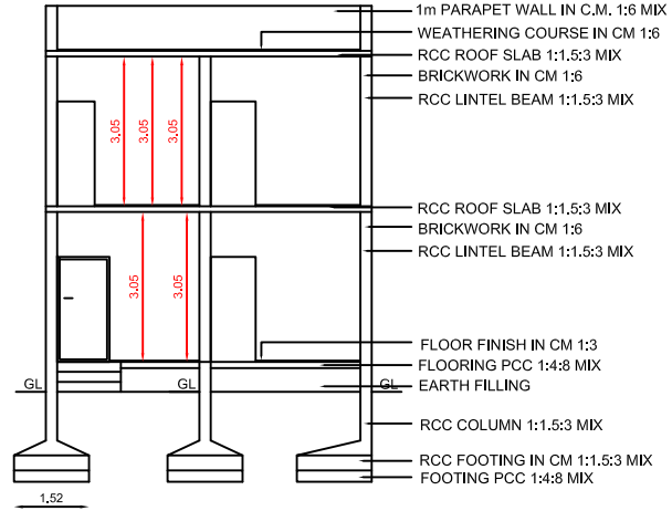
CROSS SECTION ON XY
