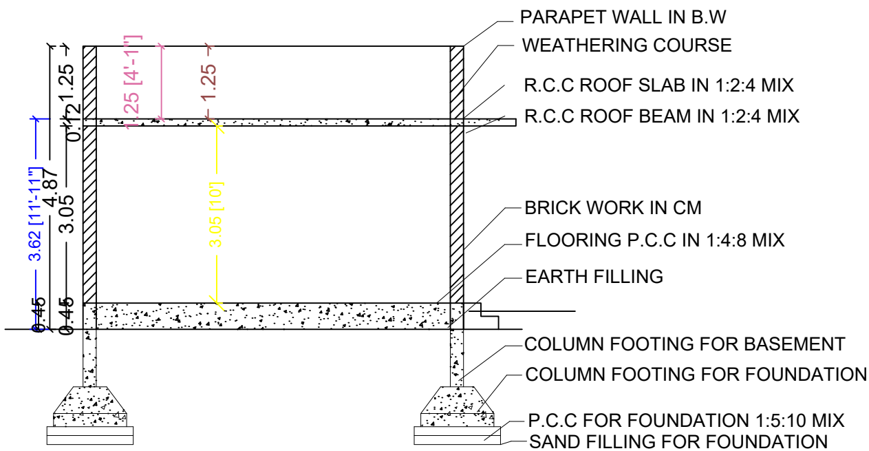
SECTION ON-AA
