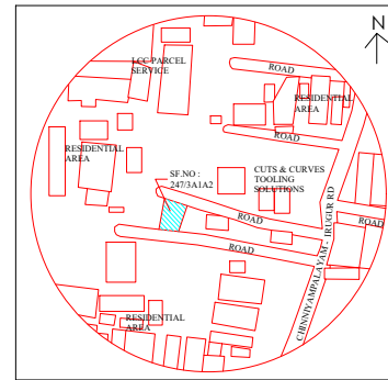
TOPO PLAN
