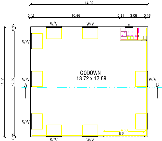
PRO.G.FLOOR PLAN
